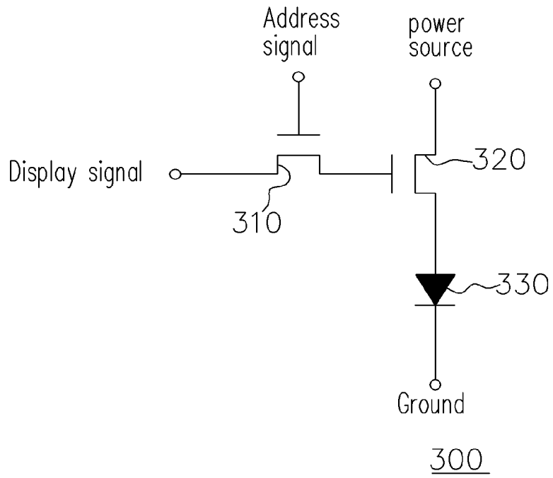
FIG. 3 (PRIOR ART)
